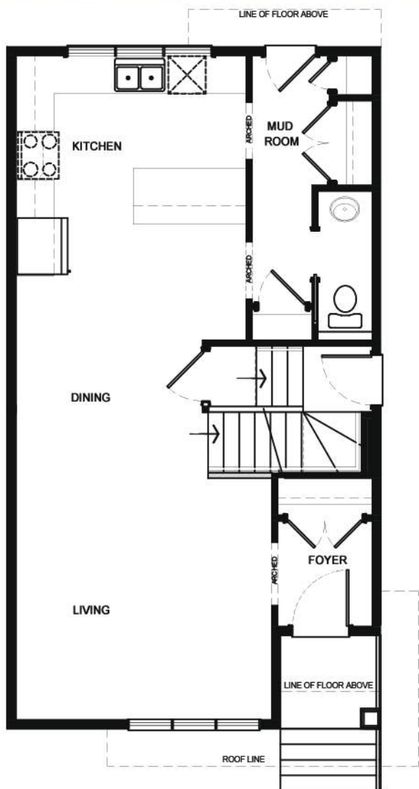
MAIN LEVEL ± 703
